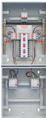
3P WITH RCD WIRING SOLUTION USING T20GH30
